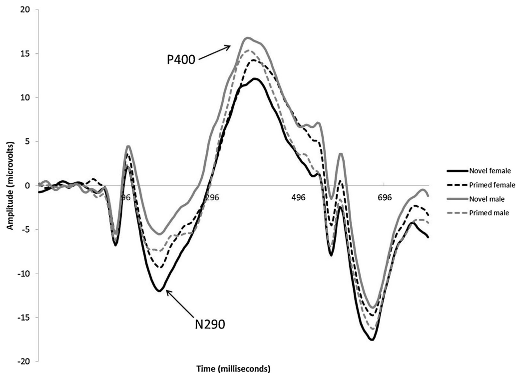
Fig. 3. Grand averaged ERP waveforms showing the N290 and P400 at posterior electrodes (collapsed across region of interest). The x-axis represents latency in milliseconds (ms) and the y-axis represents amplitude in microvolts ( \mu V ).
